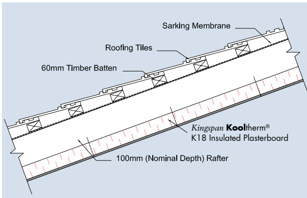
Figure 6 Side elevation - Raked ceiling with Kingspan Kooltherm ® K18 Insulated Plasterboard
