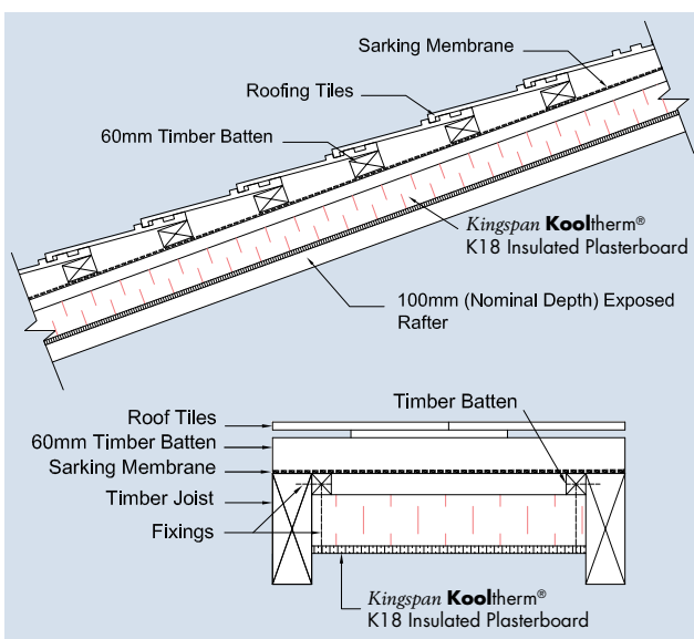
Figure 7 Side and front elevation - Raked ceiling (exposed beam) with Kingspan Kooltherm ® K18 Insulated Plasterboard
