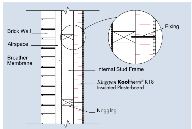
Figure 8 Side elevation - Brick veneer wall with Kingspan Kooltherm ® K18 Insulated Plasterboard
