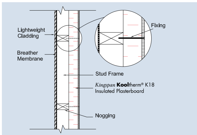
Figure 9 Side elevation - Lightweight cladded stud wall with Kingspan Kooltherm® K18 Insulated Plasterboard
